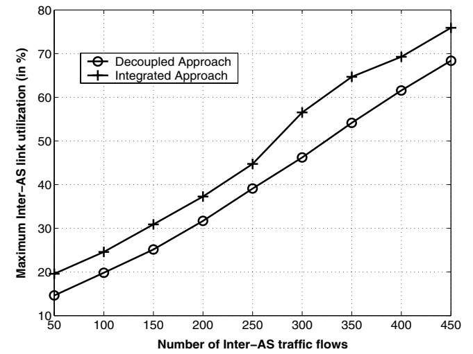
Figure 11. Evaluation of maximum inter-AS link utilization
