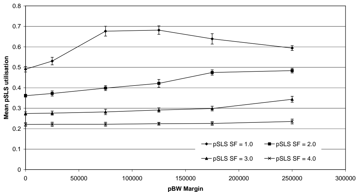
Figure 46 Mean pSLS utilisation for a range of pBW equivalence margins for the BWQA-only policy
