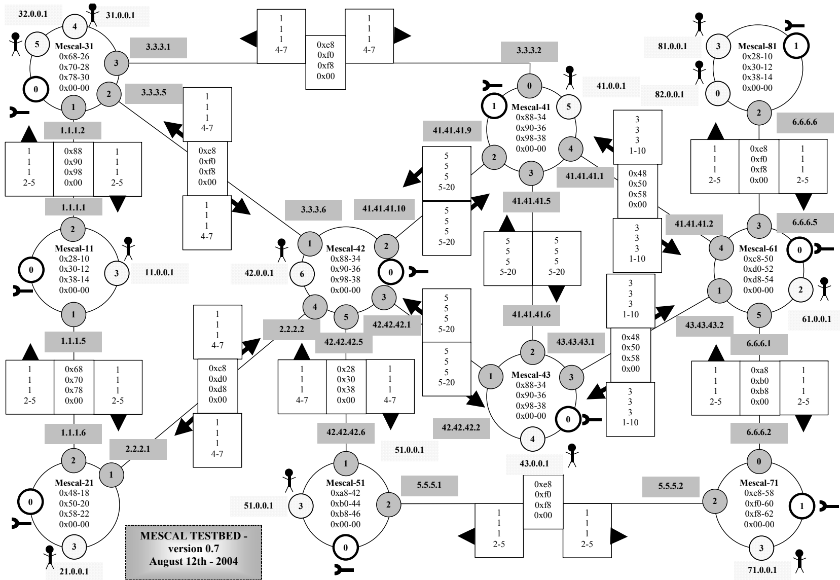
Figure 95: FTR&D Mescal testbed: detailed architecture
