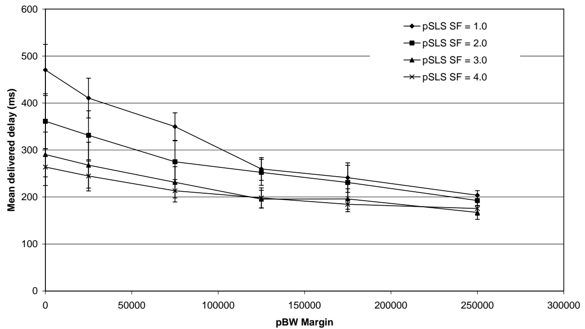
Figure 47 Mean delivered delay for various BW QA equivalence margins for the BWQA-only policy
